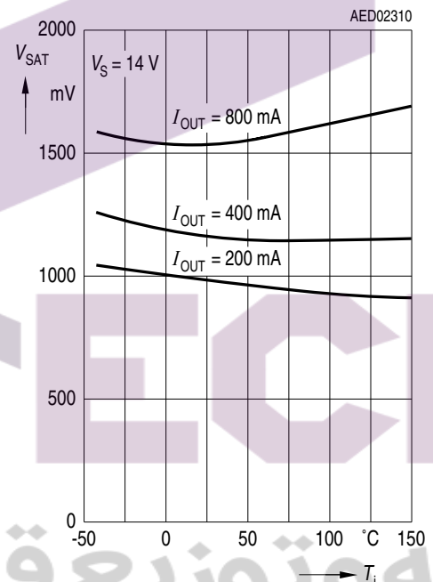
Total Drop at outputs V_{SAT} over Temperature
